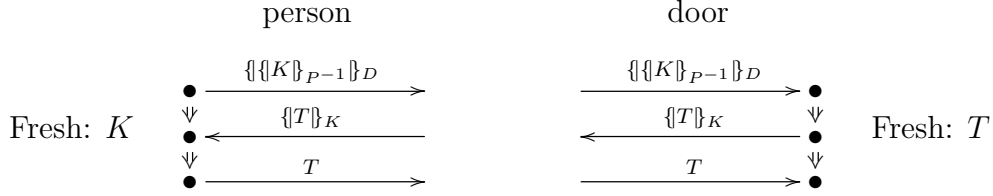
Figure 7: DoorSEP Protocol
